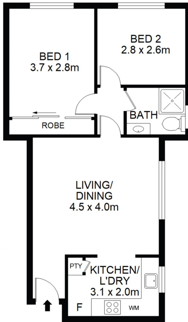
GROUND LEVEL
