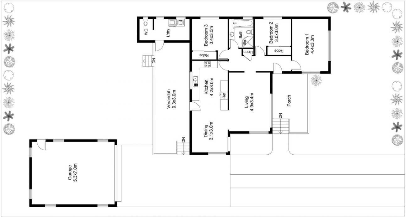
FLOOR & SITE PLAN
