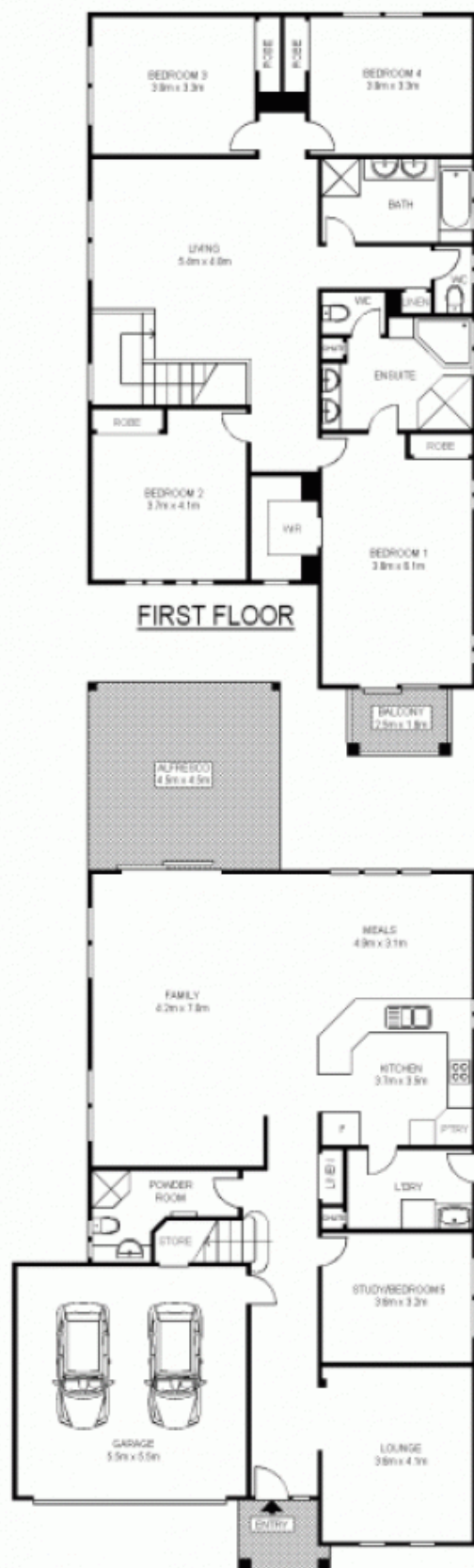
GROUND FLOOR
