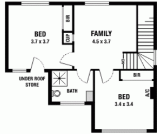
UPPER FLOOR
